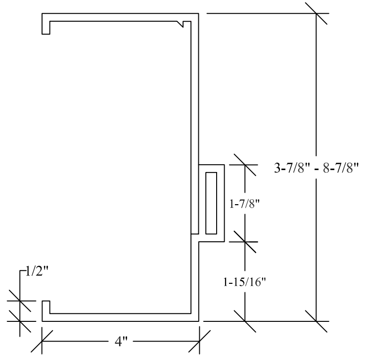
Modified 4" Head
