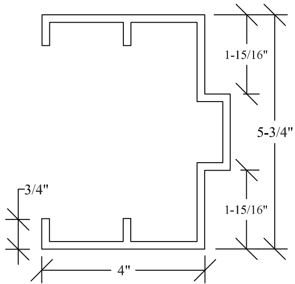
Standard 4" Head
