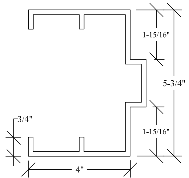
Modified 4" Head
