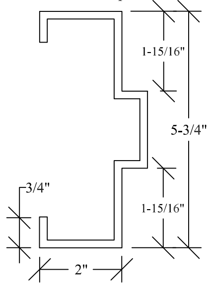
Standard Equal Rabbet
