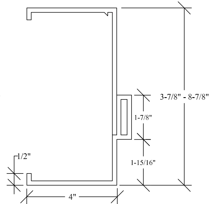
Modified 4" Head
