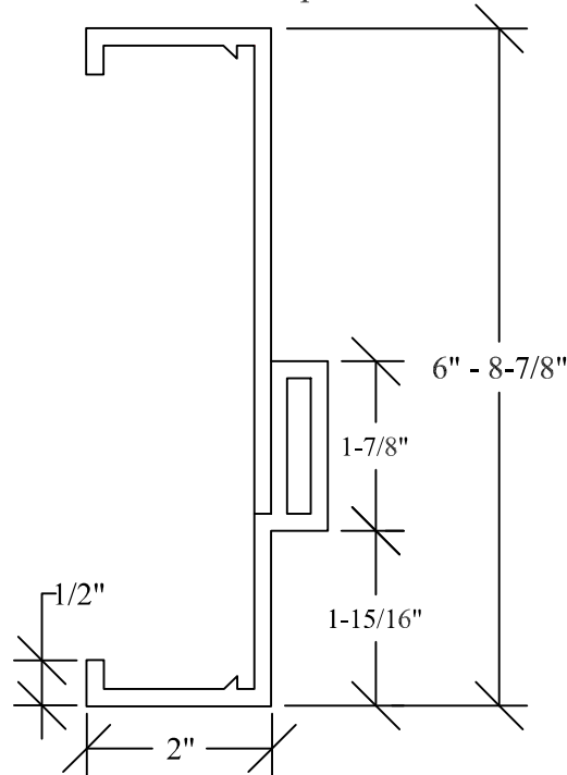
Modified Unequal Rabbet
