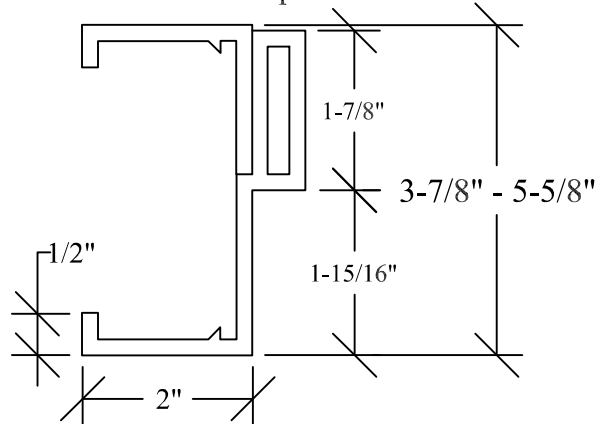
Modified Unequal Rabbet
