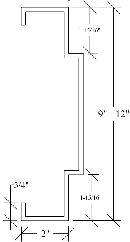
Modified Equal Rabbet
